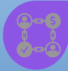
Blockchain
